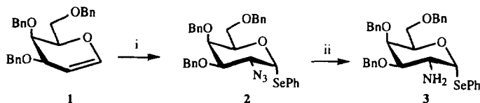
Scheme 1. Reagents: i) \text{NaN}_3 , \text{PhSeSePh} , \text{PhI}(\text{OAc})_2 , \text{CH}_2\text{Cl}_2 (40%); ii) \text{LiAlH}_4 , \text{Et}_2\text{O} (88%).
