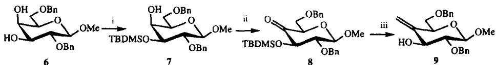
Scheme 3. Reagents: i) \text{TBDMSCl} , \text{Et}_3\text{N} , DMAP, DMF, 20 h (96%); ii) \text{PCC} , 4 Å molecular sieves, \text{CH}_2\text{Cl}_2 , 30 min (85%); iii) Tebbe reagent, THF, Pyr, -60^\circ\text{C} →rt; then aq. HF, THF, 24 h (61%).
