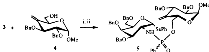
Scheme 2. Reagents: i) \text{PhPCl}_2 , \text{Et}_3\text{N} , THF; ii) t \text{BuOOH} (80% overall yield).
